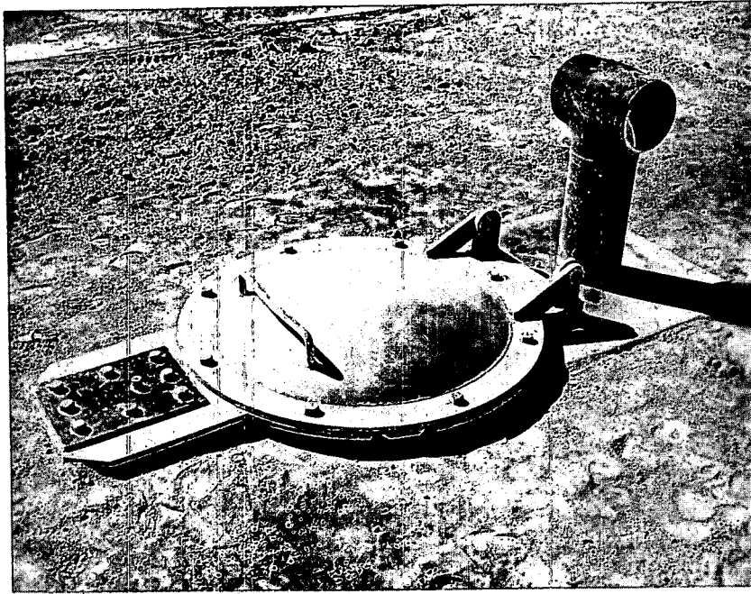
Fig. 11—Blast closure valve test plenum air-intake and access hatch after backfilling.
